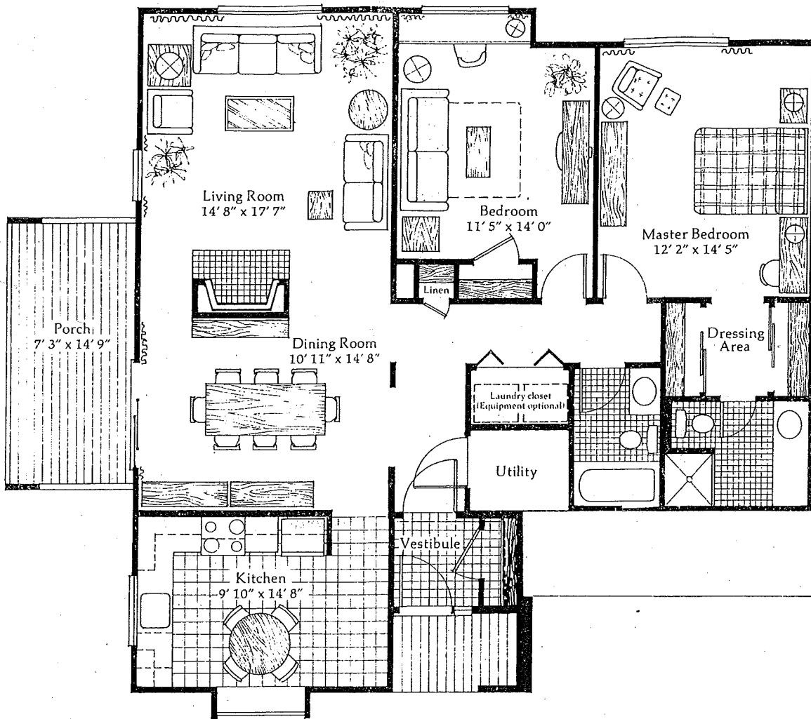
First Level
