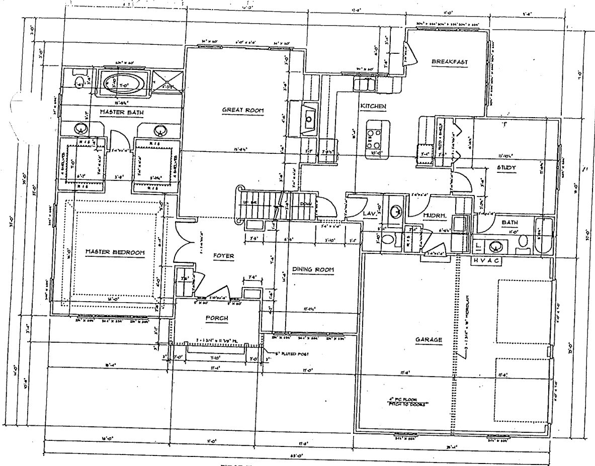
FIRST FLOOR PLAN 1310 S.F. SCALE: 1/8" = 1' - 0"
