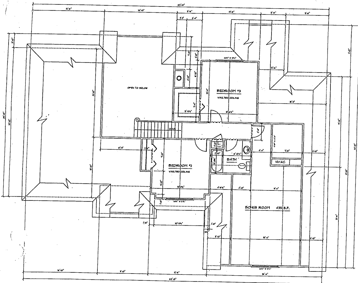
SECOND FLOOR PLAN 530 S.F. SCALE: 1/8" = 1' - 0"
