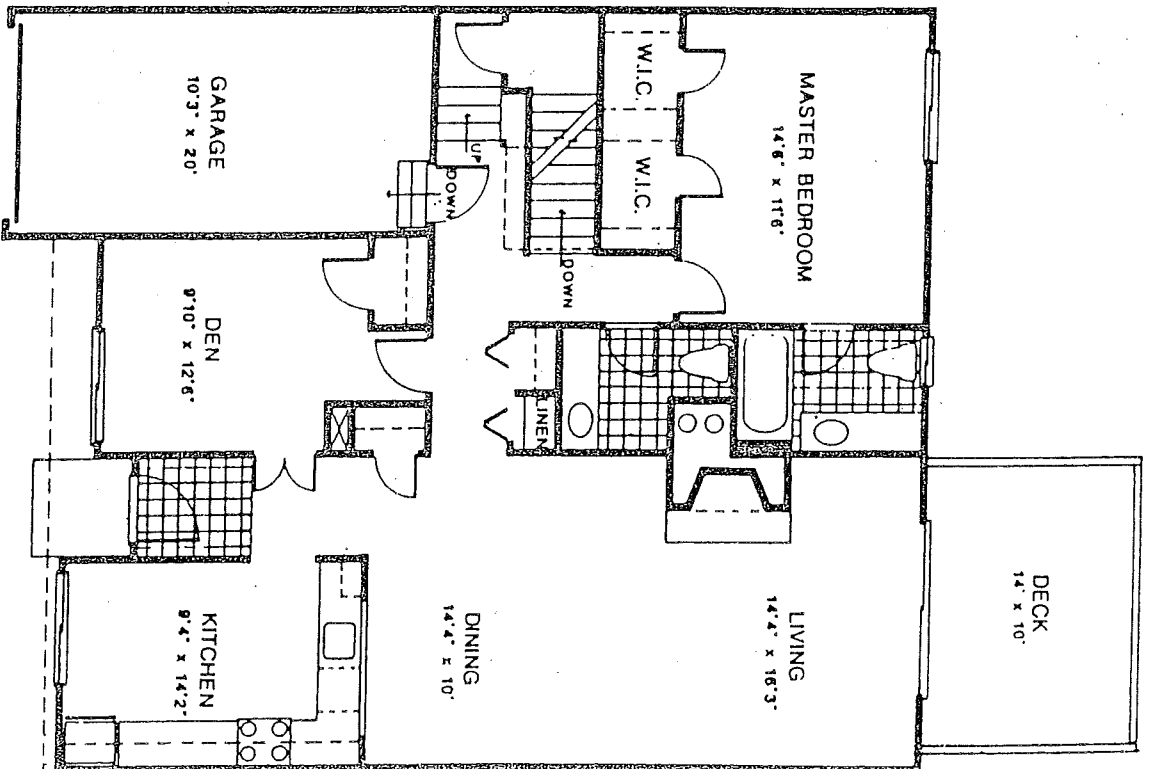
ENTRY LEVEL
